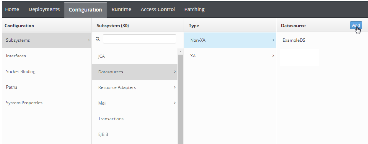
Figure 17: Configuring a JNDI connection
