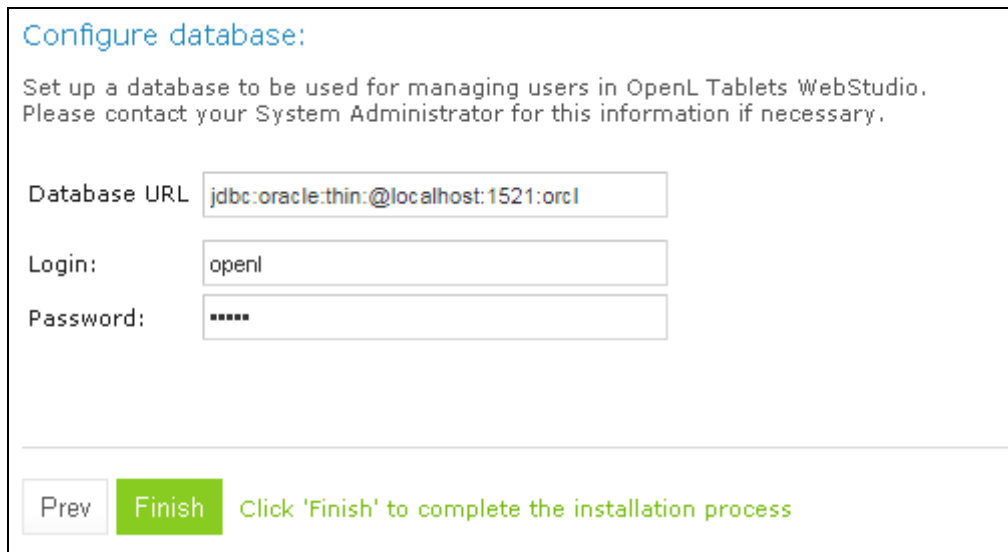
Figure 4: Creating a connection to the Oracle database in the installation wizard
