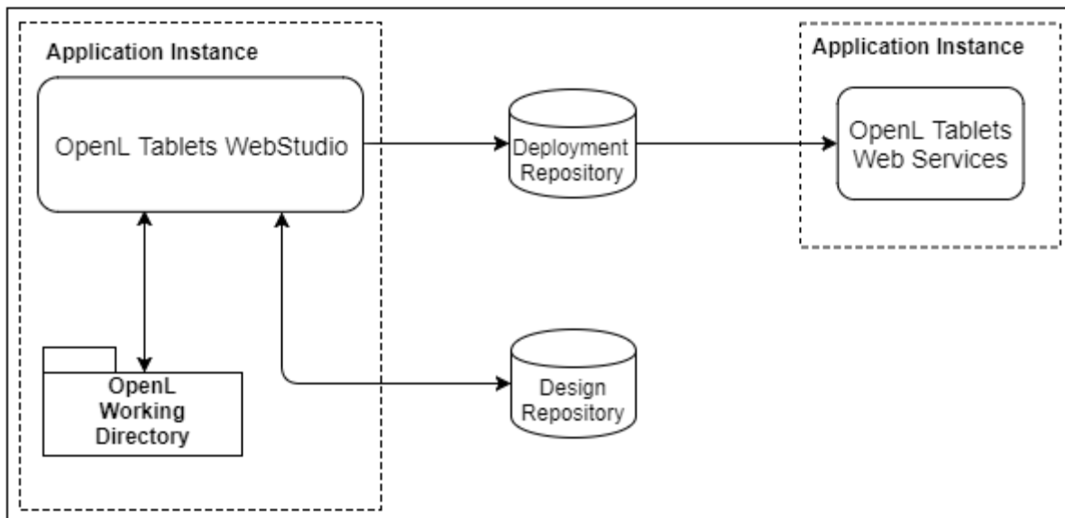
Figure 19: OpenL Tablets WebStudio and OpenL Tablets Rule Services deployment
