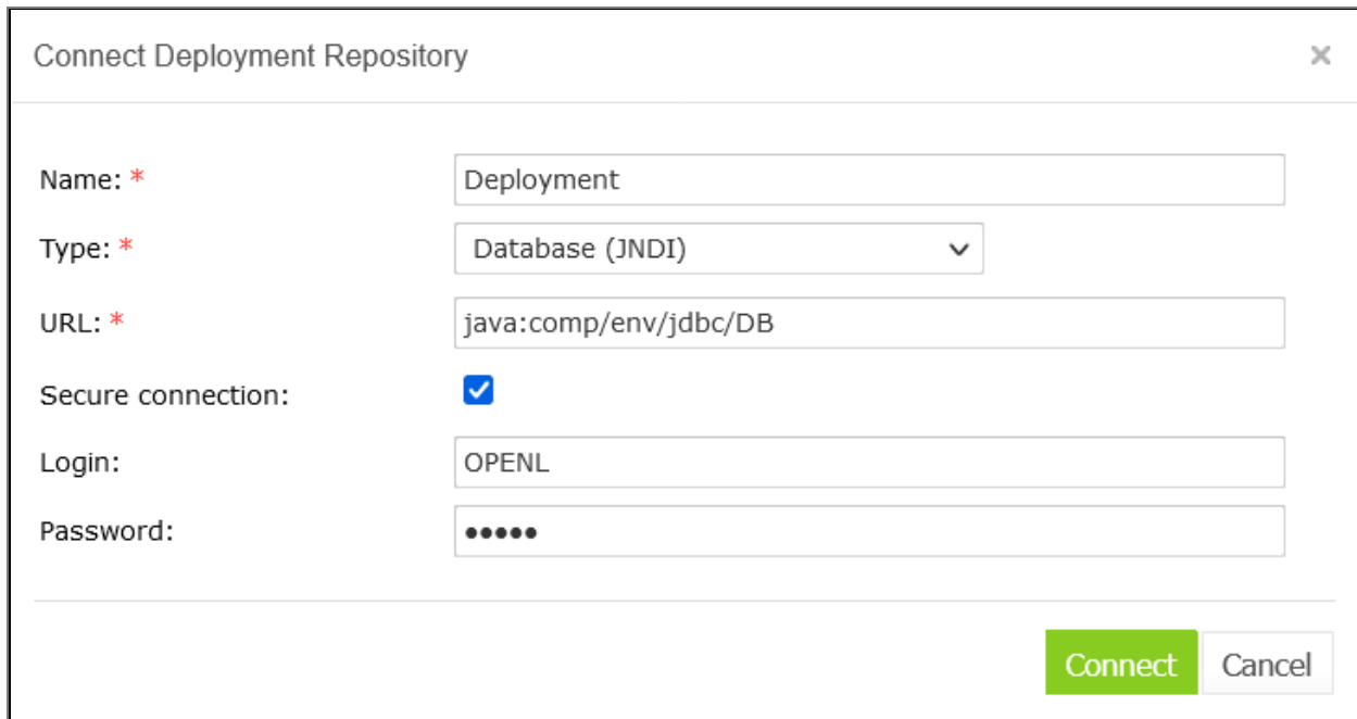
Figure 10: Setting up JNDI connection with installation wizard
