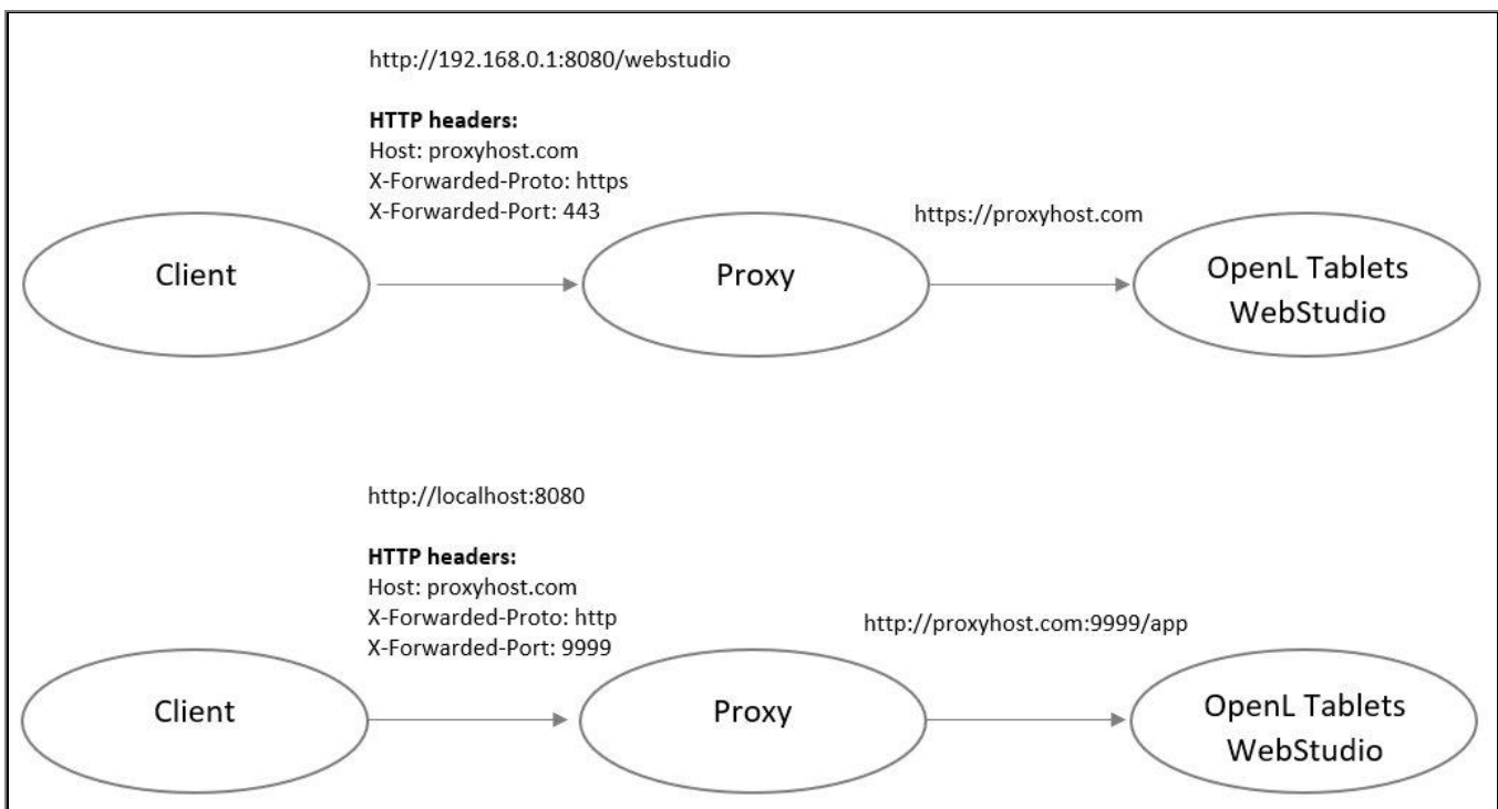
Figure 11: Connecting to OpenL Tablets WebStudio via proxy
